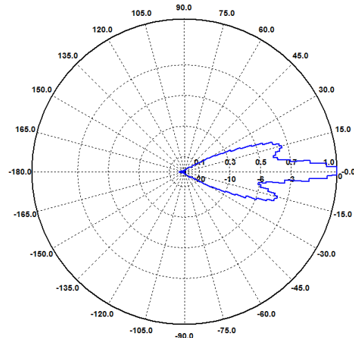
H-Ebene / H-Plane 6 GHz
