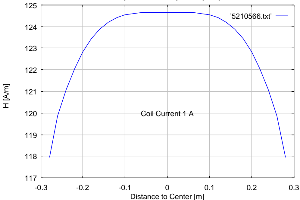
Spulenabstand 0.566 m Coil Distance 0.566 m
