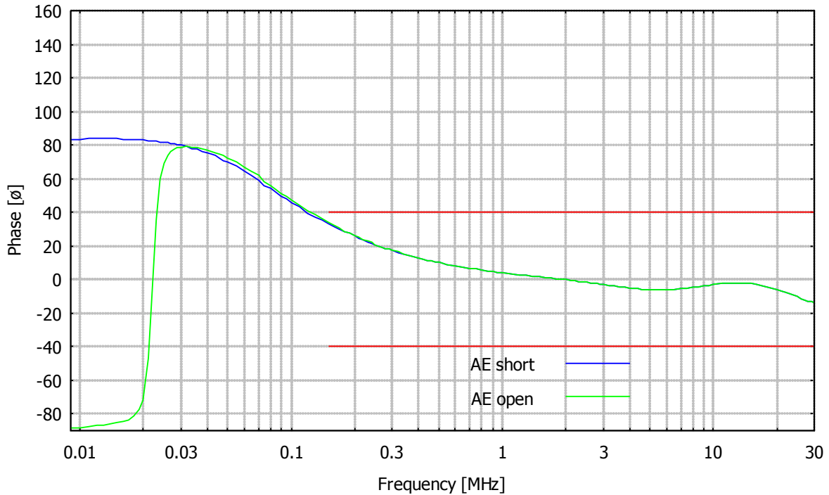
Phase an den Prüflingsklemmen - differential mode, (Kalibrieradapter erforderlich), BNC mit 50 \Omega Abschluss Phase at EuT-Terminals (Calibration adapter required), BNC-Port is terminated with 50 \Omega
