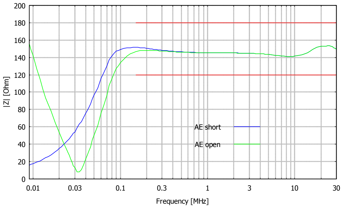
Impedanz an den Prüflingsklemmen - common mode, mode A, B (Kalibrieradapter erforderlich), BNC mit 50 Ω Abschluss Impedance at EuT-Terminals (Calibration adapter required), BNC-Port is terminated with 50 Ω
