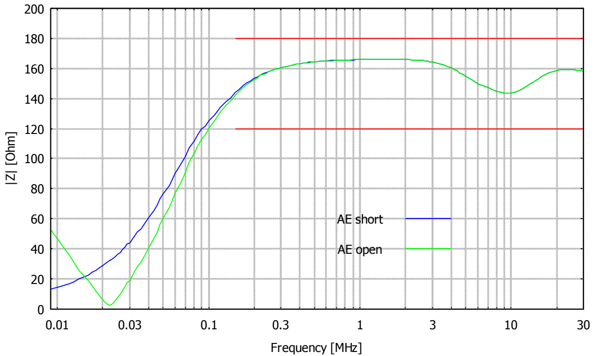
Impedanz an den Prüflingsklemmen - differential mode (Kalibrieradapter erforderlich), BNC mit 50 \Omega Abschluss Impedance at EuT-Terminals (Calibration adapter required), BNC-Port is terminated with 50 \Omega
