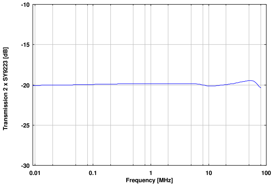
Abb. 1 Transmission zweier SY9223-135 an EuT verbunden Fig. 1: Transmission of two SY9223-135 connected at the EuT port
